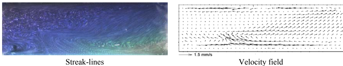
Figure 3. Transition front observed 1min after temperature reversal; \alpha = 10^\circ , \Delta T = 6K .
