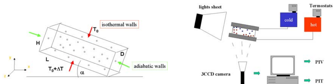
Figure 1. Schematic of the experimental apparatus: (a) – cavity, (b) – basic elements of the experimental rig
