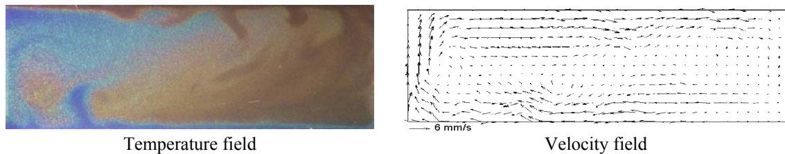
Figure 2. Snap-shots of the temperature and velocity fields observed for the up-slope convection in the cavity; \alpha = 20^\circ , \Delta T = 6K .
