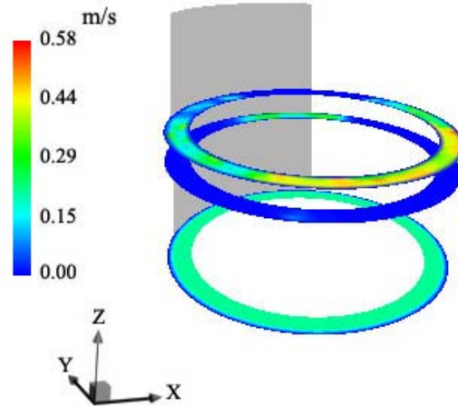
Fig. 3. Contours of particle phase velocity at three different elevations calculated during a numerical simulation. Here \Gamma = 1.30 , the mean height = 5\text{ cm} , A = 0.534\text{ cm} and frequency f = 7.78\text{ Hz} .
