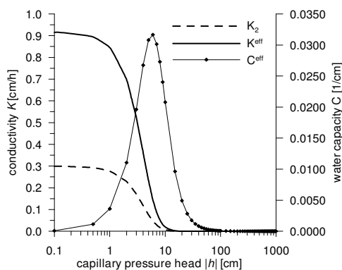
Fig. 3. Hydraulic parameters of the soil
