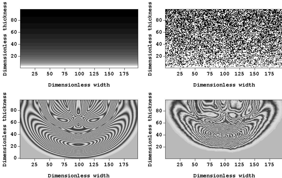
Fig.1. Density distributions and wavefronts in metal-ceramic composite for different models.
