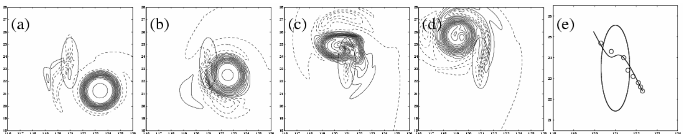
Figure 2 Comparison of shallow water simulation and the dynamic model results of vortex evolution over topography.
