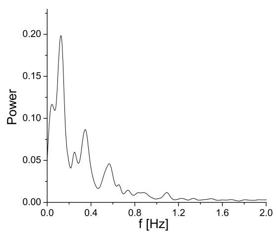
Figure 5. Power spectrum of velocity fluctuations in the center of the vessel
