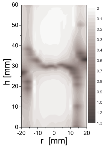
Figure 4. Turbulence degree belonging to the flow in Fig. 3
