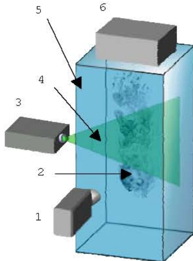
Fig.1. The experimental setup: 1) a camera, 2) a cloud during mixing, 3) a laser, 4) laser sheet, 5) a cloud chamber, 6) a small chamber with the droplet generator inside .
