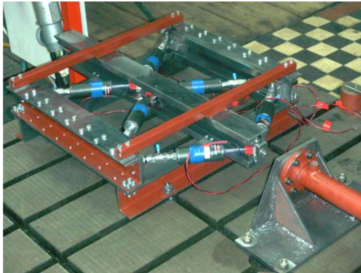
Fig.3. Experimental setup
